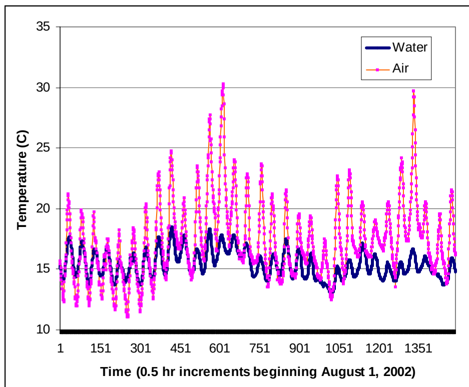
Figure 4. Temperature variability for August 2002 on Cowlitz River at Kelso
