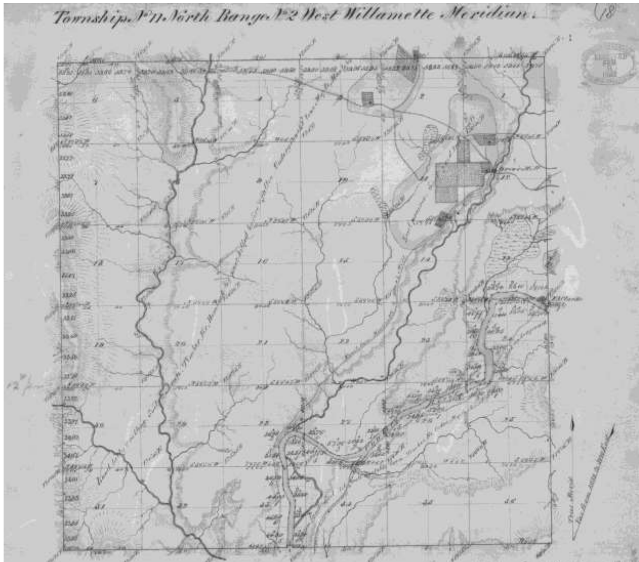
Figure 28. Historical GLO map of the Cowlitz River from Olequa Creek to near Salmon Creek (USBLM 1884)
