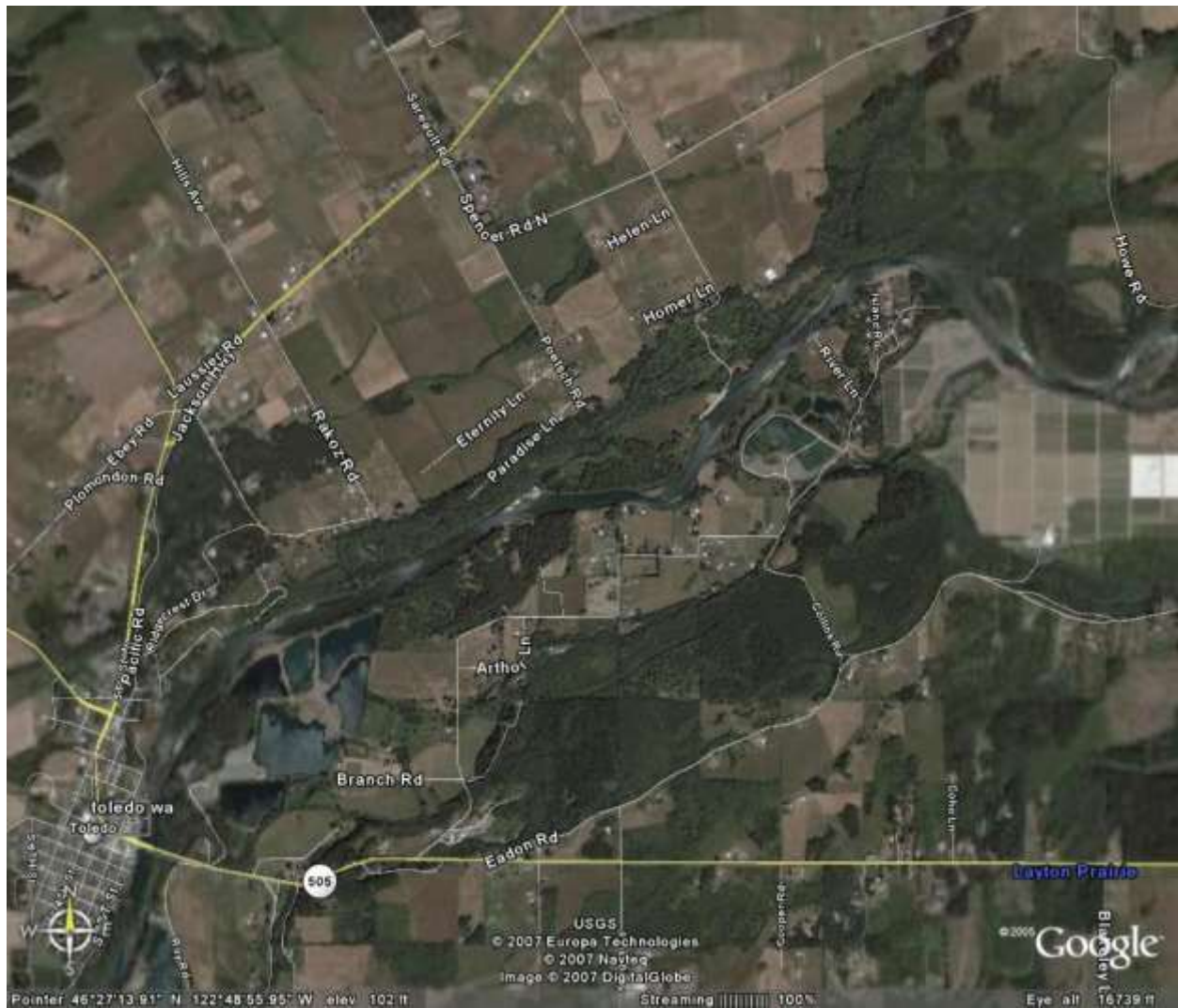
Figure 37. Current Aerial of the Cowlitz River Upstream of Toledo (Google Earth 2007)
