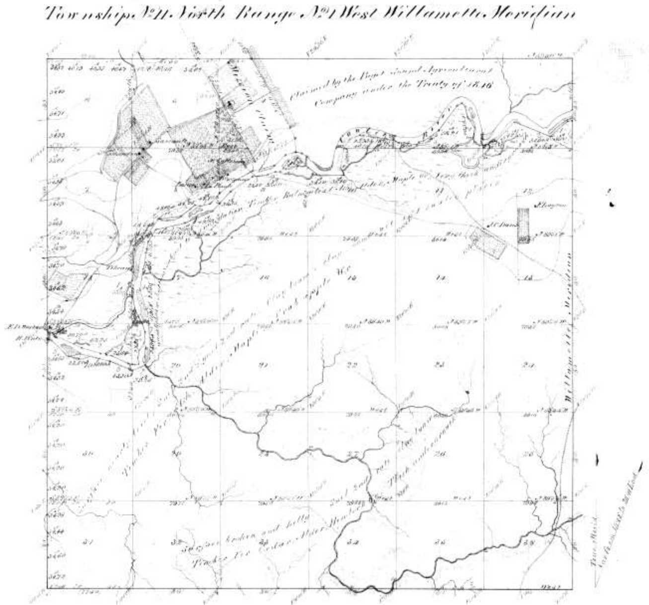
Figure 35. Historical GLO map of the Cowlitz River near Toledo
