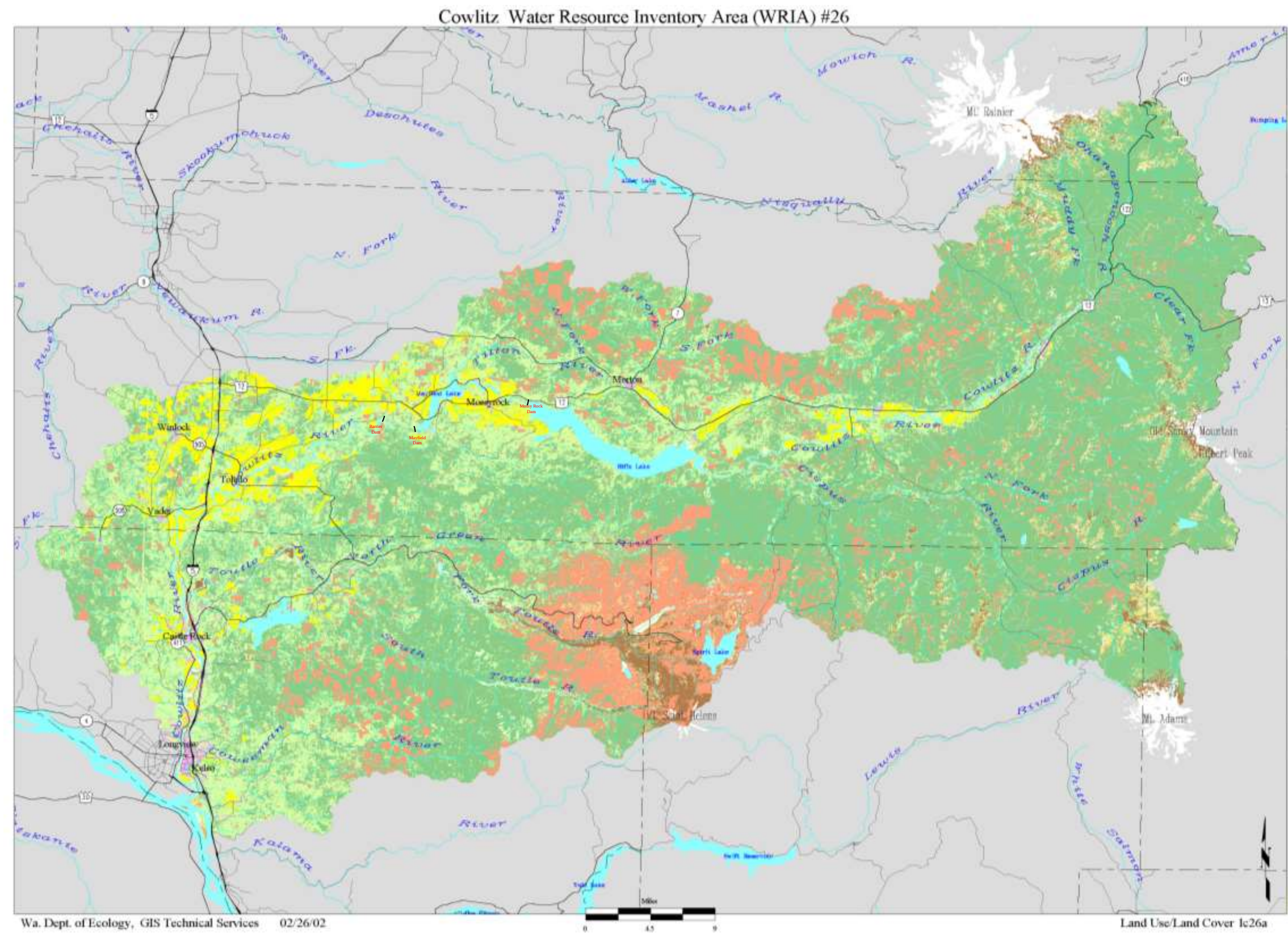
Figure 2. Cowlitz River Watershed (from WDOE 2002).
